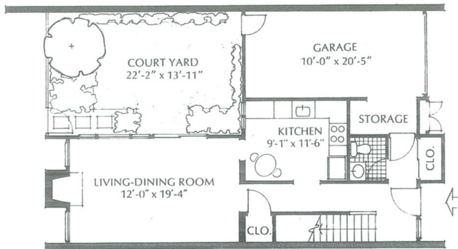
GROUND LEVEL PLAN
